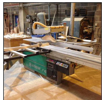
Altendorf F45 Panel Saw
